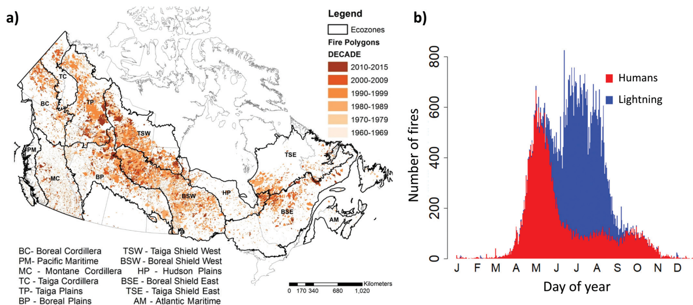
Fig. 1. (a) National distribution of large fire (>200 ha) polygons in Canadian ecozones. Figure adapted from Hanes et al. 2019. The base map was made in ArcGIS and includes the National Fire Database polygon data and Canadian ecozone polygons. (b) Stacked bar graph showing the number of new human- and lightning-caused fire occurrences ( \geq 2 ha) for each day of the year from 1959 to 2018. Figure adapted from Coogan et al. 2020. [Colour online.]
