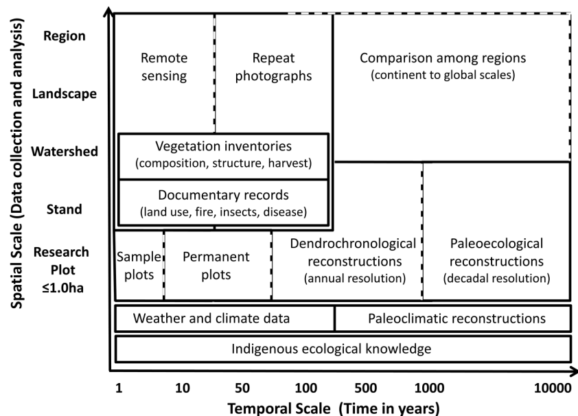
Fig. 2. Conceptual model of the spatiotemporal domains of research approaches used to characterize fire regimes.
